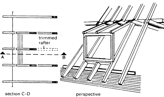
7 Dormer window in a purlin roof
